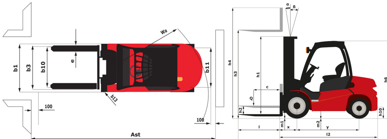
MI-X 70 D - Dimensional drawing
