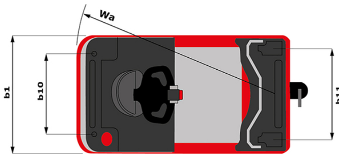
CT 40 - Dimensional drawing
