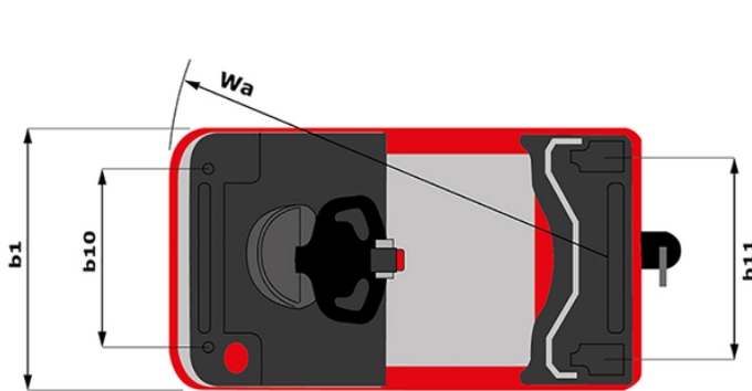
CT 40 - Diagrama dimensional
