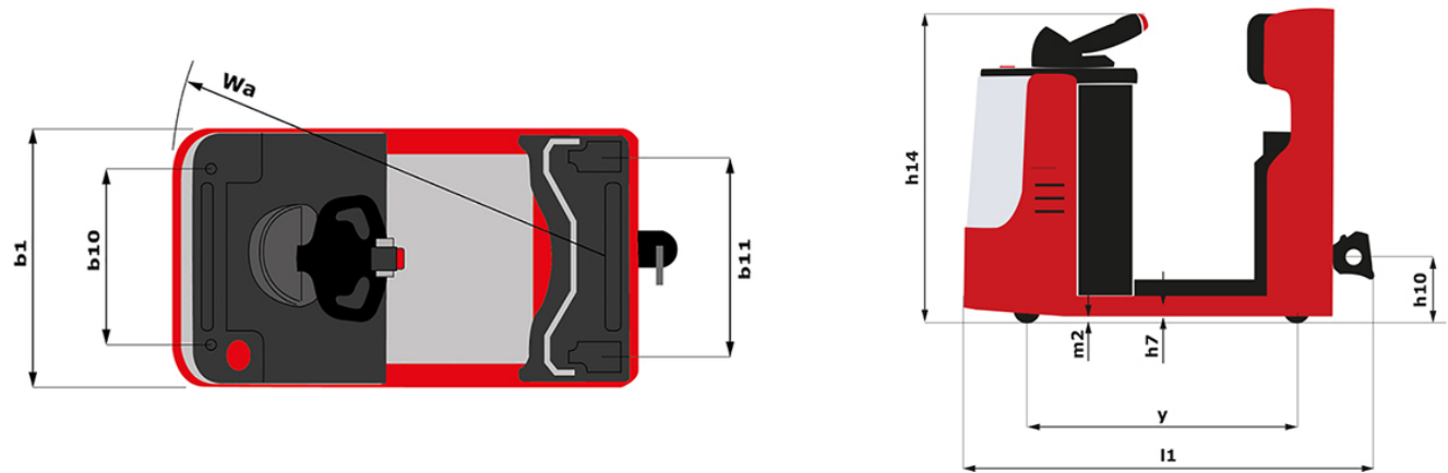
CT 40 - Diagrama dimensional
