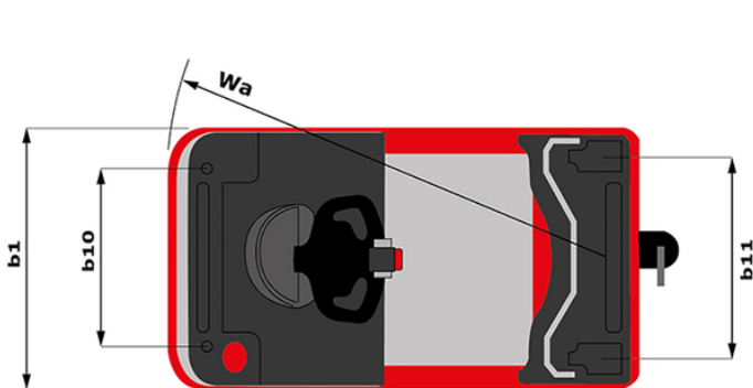
CT 40 - Diagrama dimensional
