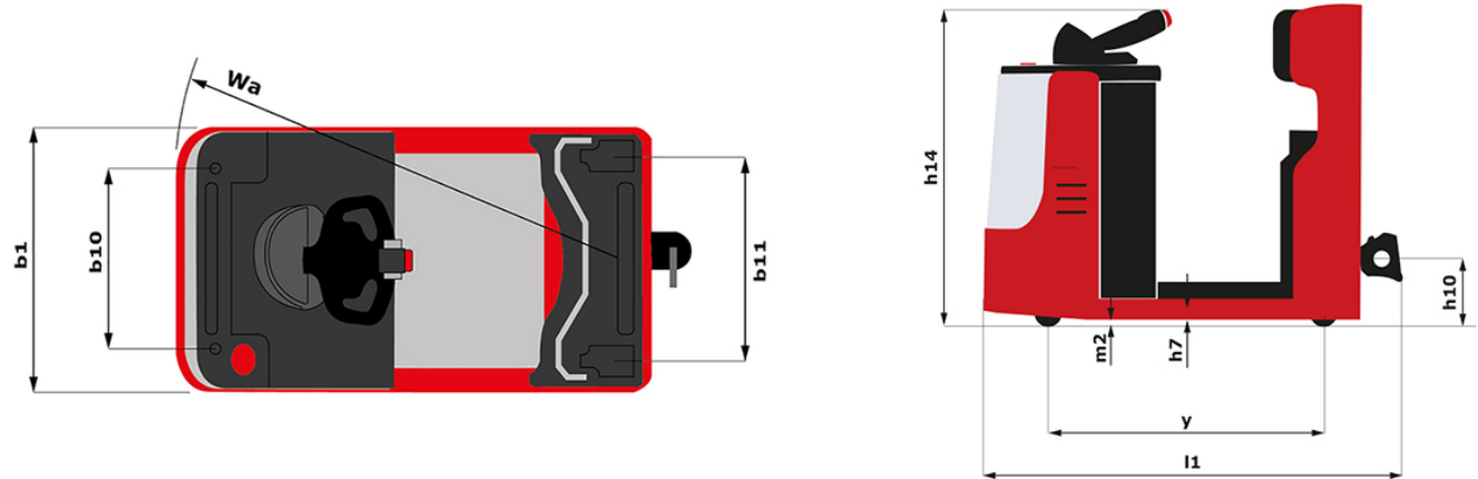
CT 40 - Dimensional drawing
