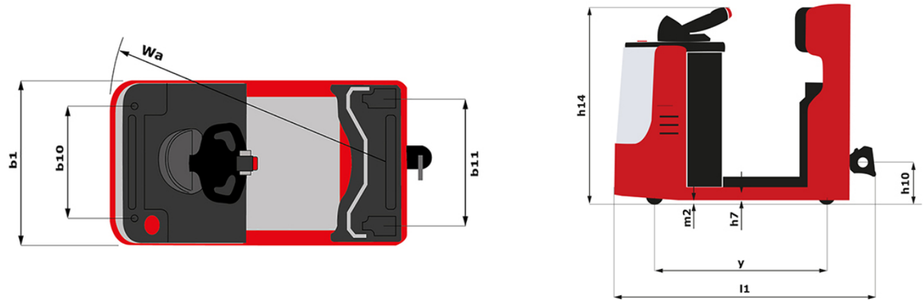
CT 30 - Diagrama dimensional
