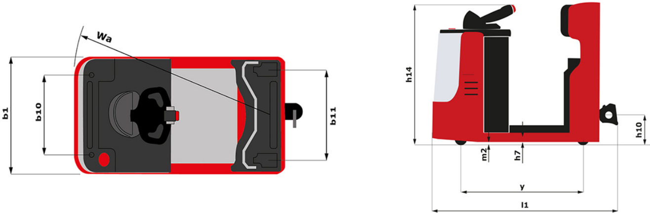
CT 30 - Dimensional drawing
