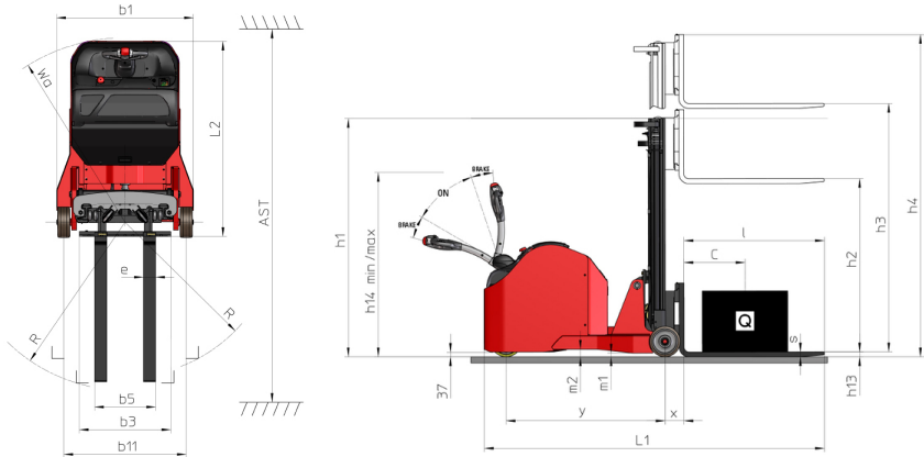
ES-C 720 - Dimensional drawing
