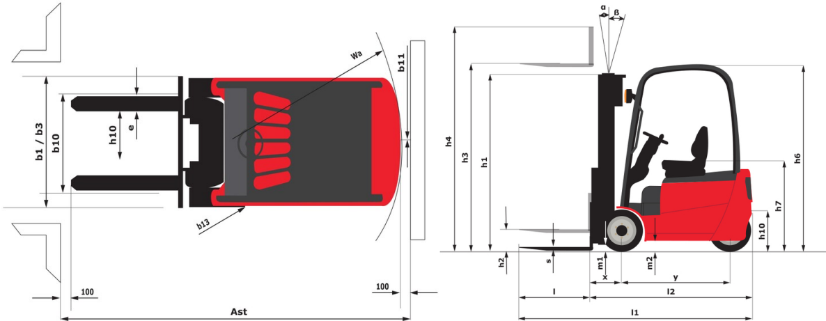
ME 445 - Diagrama dimensional
