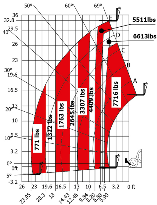
Machine on tires with forks Imperial
