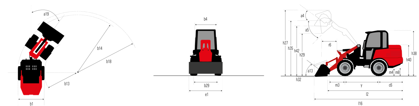
MLA 4-50 H - Dimensional drawing
