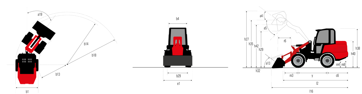
MLA 4-50 H-C - Dimensional drawing
