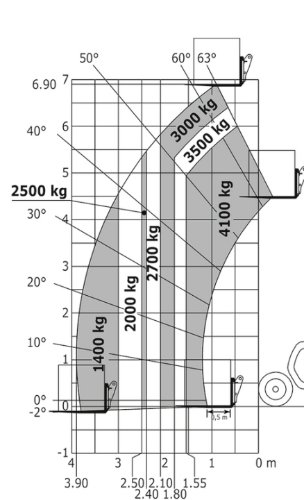
Machine on tyres with forks Metric
