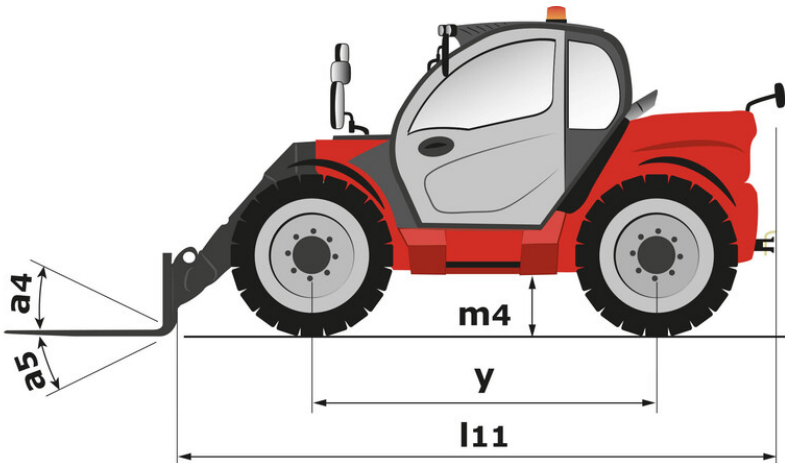
MLT 1041-145 PS+L - Dimensional drawing
