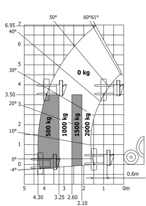
Machine on tyres with tyre handler TH 33 (Metric)
