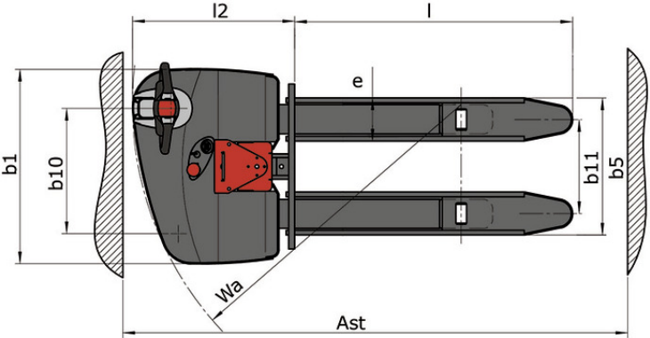
Stacky 14 - Dimensional drawing
