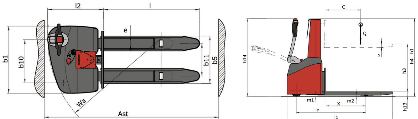
Stacky 14 - Dimensional drawing
